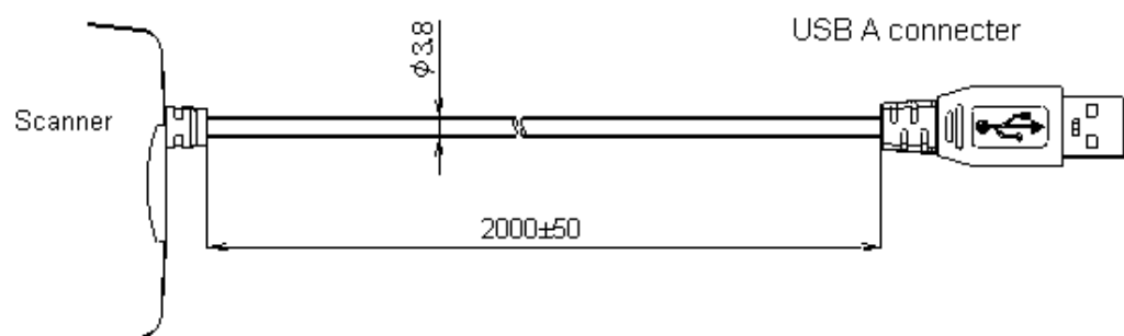
Figure 23: USB cable
