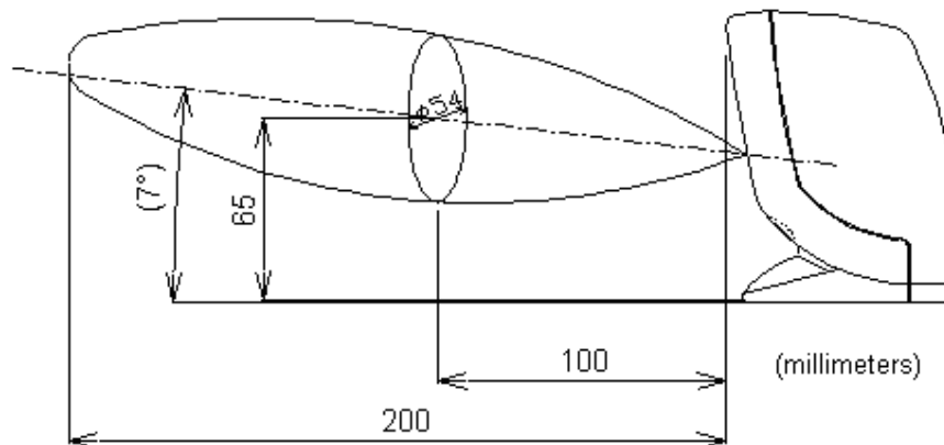
Figure 30: Auto-trigger detection area
