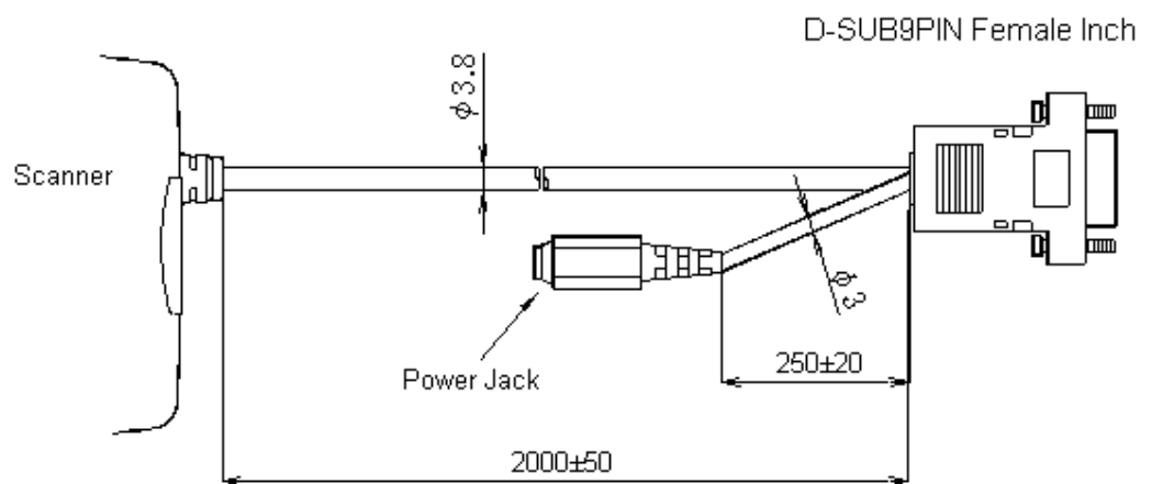
Figure 22: RS-232C cable
