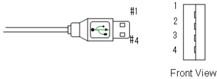
Figure 17: USB "A" connector
