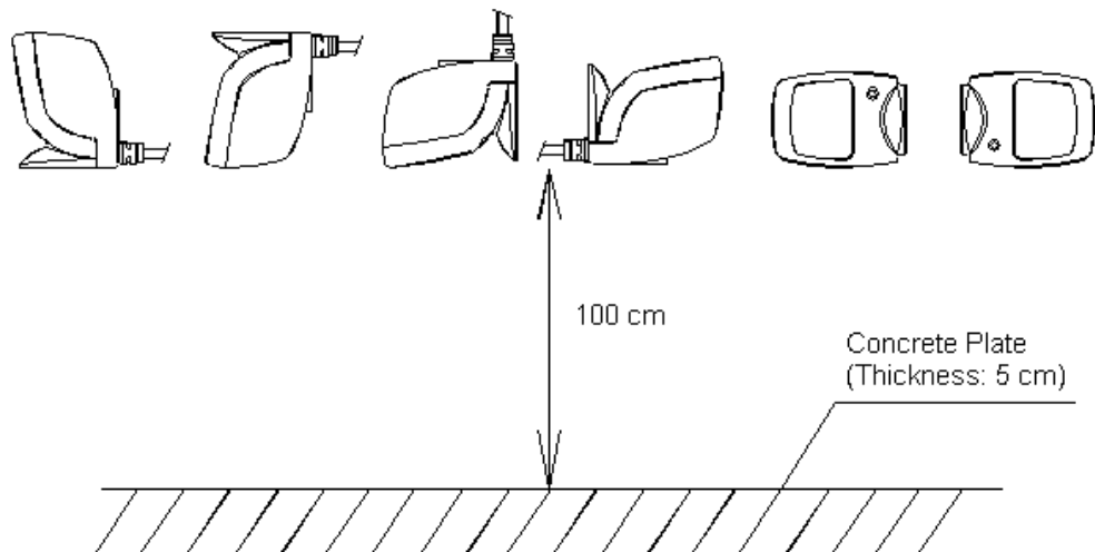
Figure 28: Drop test
