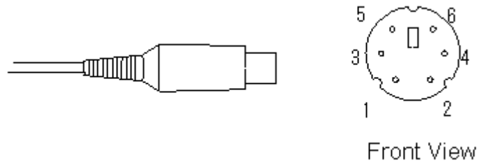
Figure 21: Wedge connector (DOS/V side)
