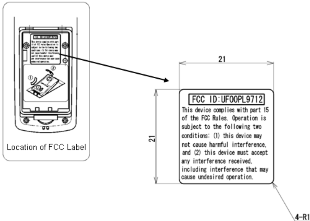
Figure 8: FCC label
