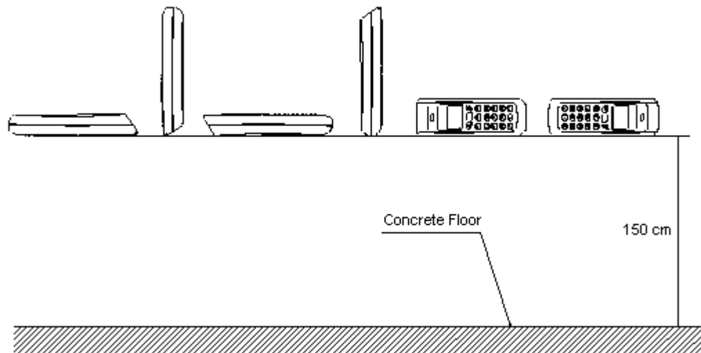
Figure 11: Shock test
