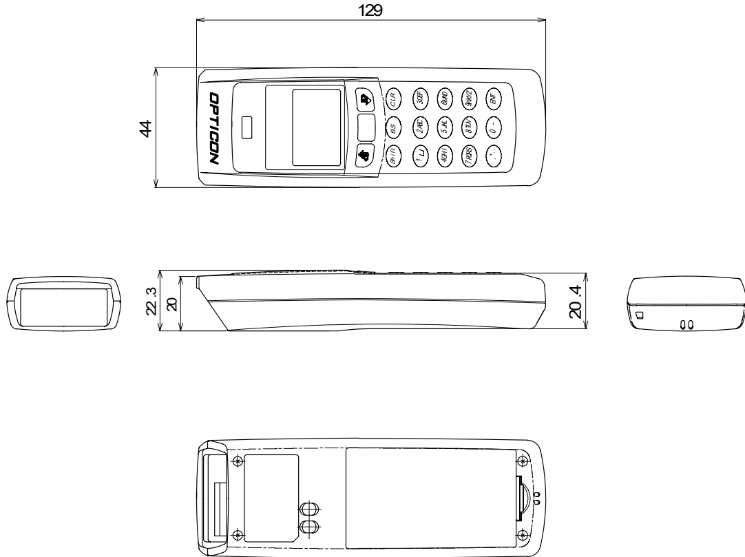
Figure 12: Mechanical drawing
